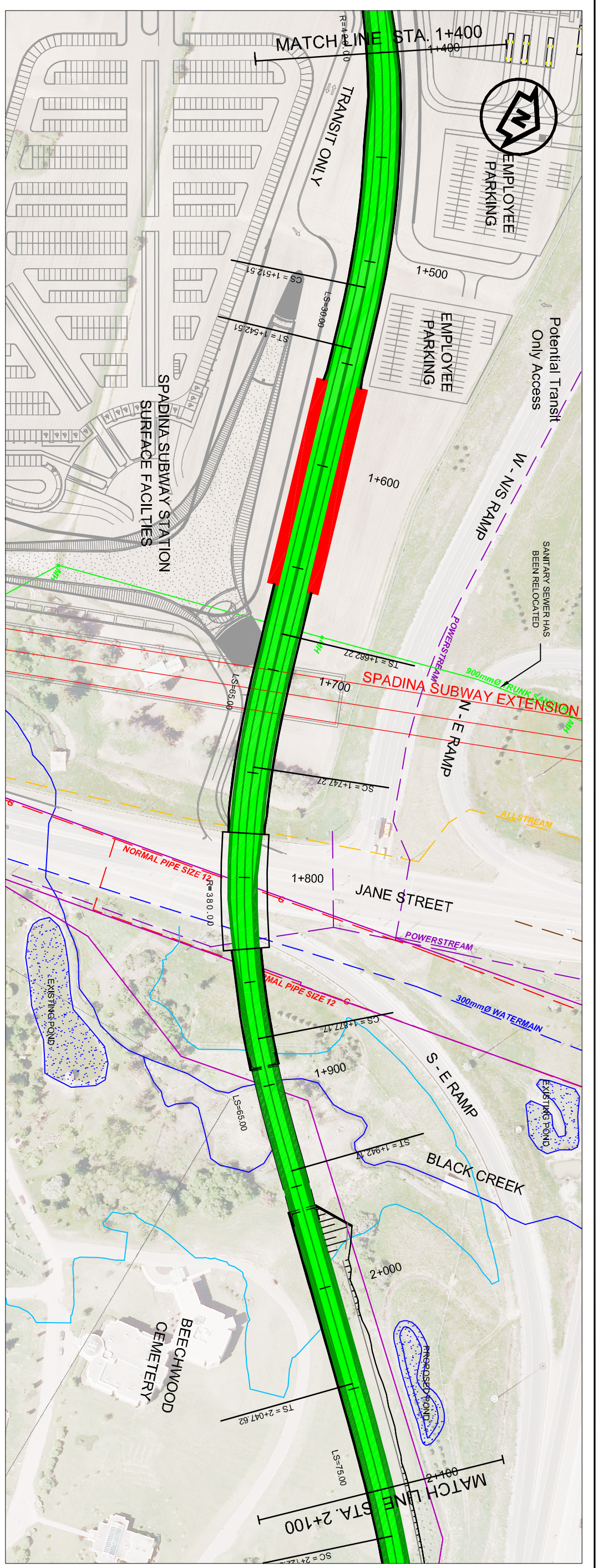
HORIZONTAL AND VERTICAL ALIGNMENT OF THE SPADINA SUBWAY EXTENSION 407 STATION AS PROVIDED BY TTC (SEPTEMBER 2010)
